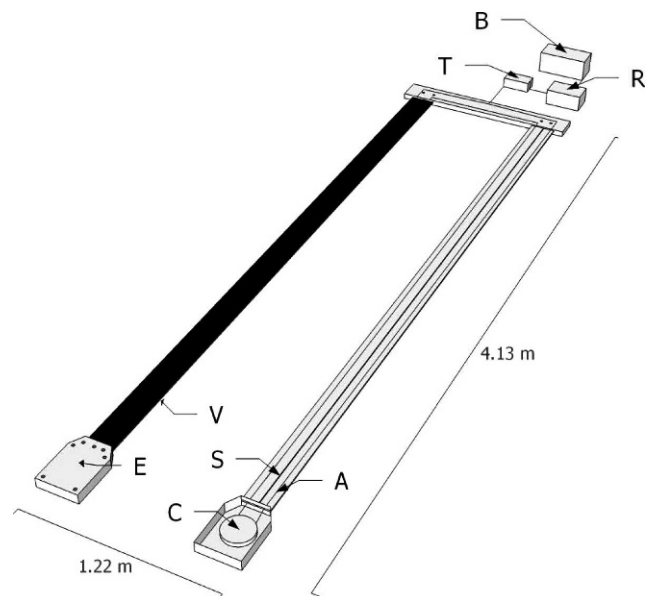
FIG. 1. Schematic representation of a boat-mounted radio frequency identification (RFID) antenna system consisting of an antenna with a single continuous 12-gauge stranded copper wire (A) with 2 antenna coils (C) encased in a protective high-density polypropylene housing (E) and 2 flexible vinyl-coated polyester droppers (V) with a 9-mm-diameter Spectra® rope (S). The antenna was connected to a low-frequency half-duplex RFID reader (R) via the antenna tuner (T) and was powered by a 12-V direct-current battery (B).
