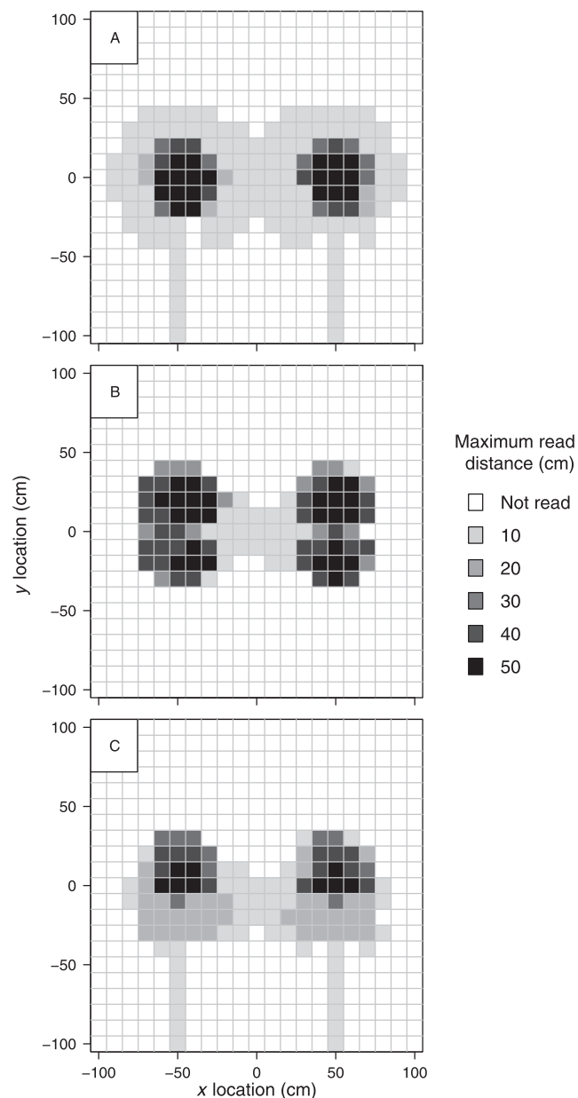
FIG. 3. Maximum detection distance tested underwater with a 32-mm half-duplex passive integrated transponder (PIT) tag for vertical (A), horizontal (B), and 45° (C) tag orientations in relation to the antenna coil. The origin of the grid (0,0) represents the midpoint of the x -axis between the antenna coils that was centered on the coils in the y -axis orientation.
